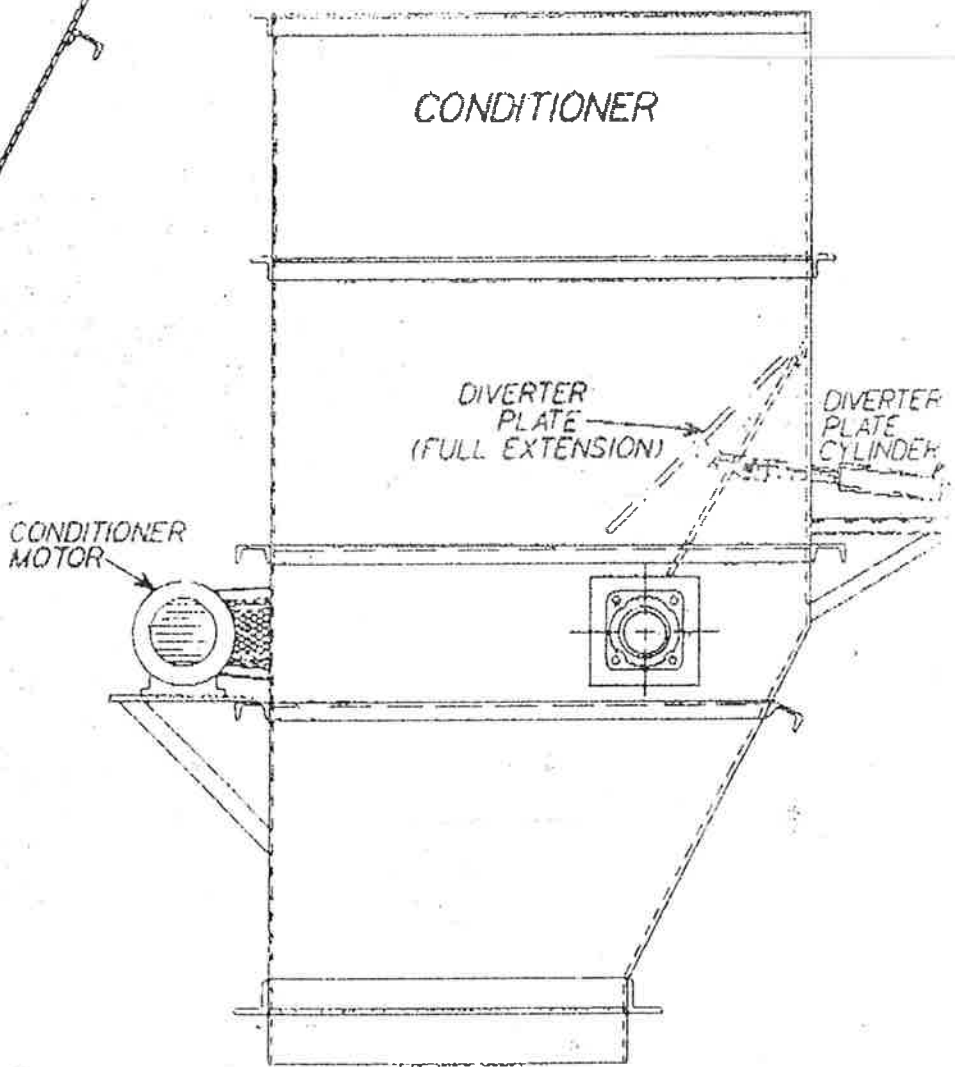
SIDE VIEW
